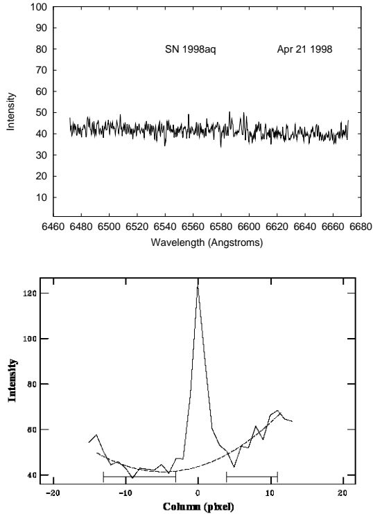
Fig. 4. Up: High resolution spectrum of SN 1998aq in the H\alpha region obtained at 1 week before maximum. No significant sign of the hydrogen Balmer-alpha line is present. Bottom: Subtraction of background contamination from the spectrum.
